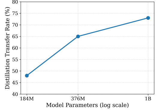
Figure 3: Distillation transferability as a function of student model capacity. Smaller students still benefit from distillation, but transferability drops as the teacher-student capacity gap increases.
